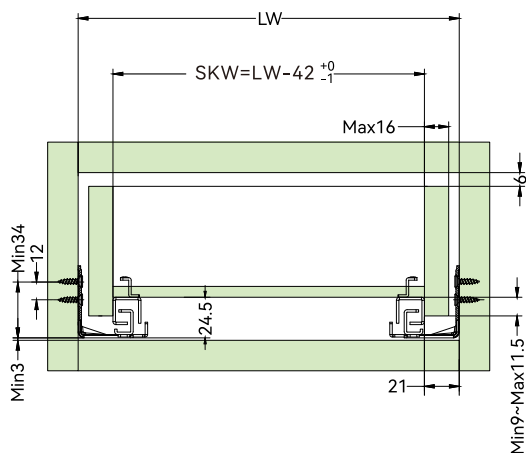
Screw positions of the slides(mm)
